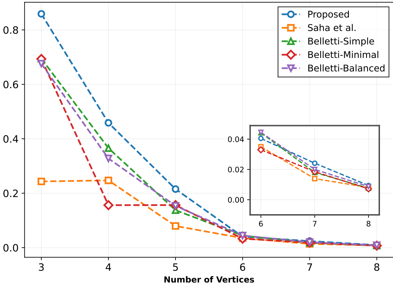
Total Probability of the Desired Solution States
