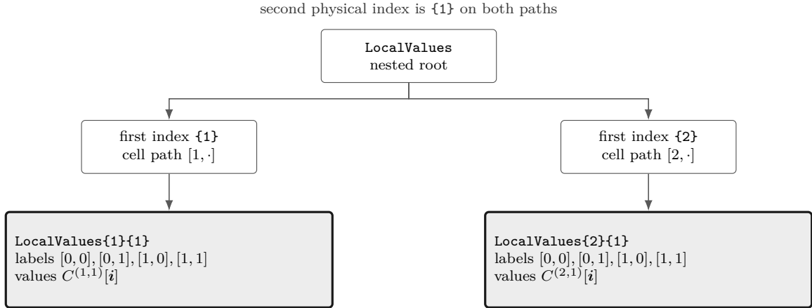
Figure 3.1: Nested cell-wise storage for a two-parameter, degree-one object on \{[0 \ 1 \ 2], [10 \ 20]\} . There are two physical cells, [1, 1] and [2, 1] . Each leaf is a flat local coefficient cell in 1b1s order: [0, 0] , [0, 1] , [1, 0] , [1, 1] .
