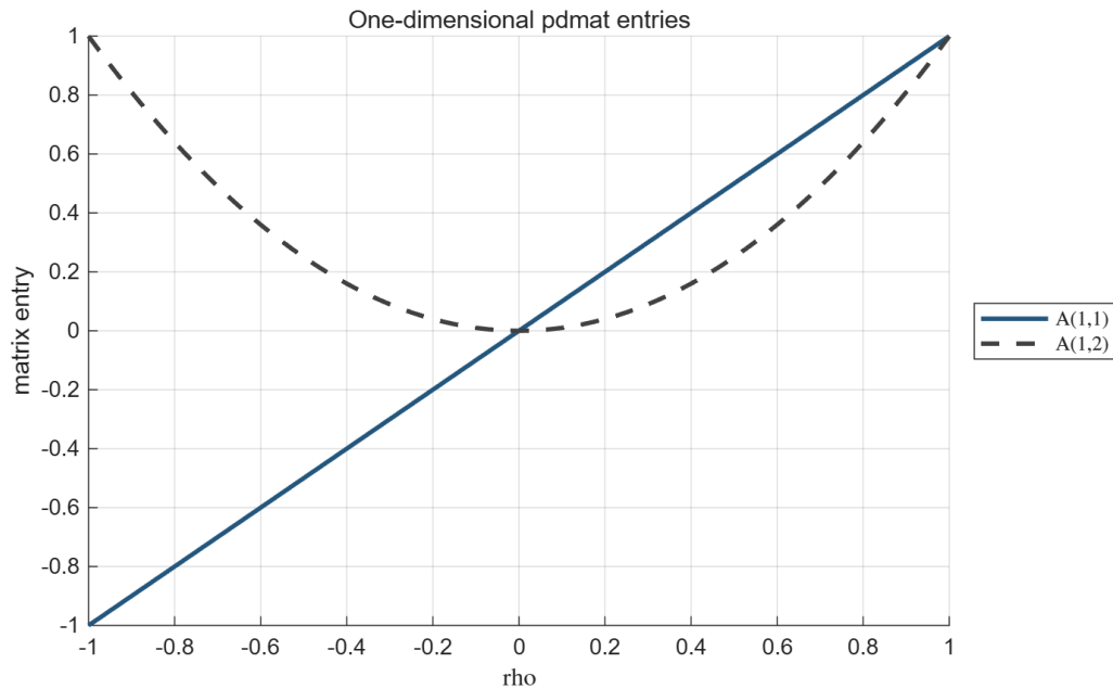
Figure 5.1: Result of the one-dimensional source above. The method returns one line handle per matrix entry.
