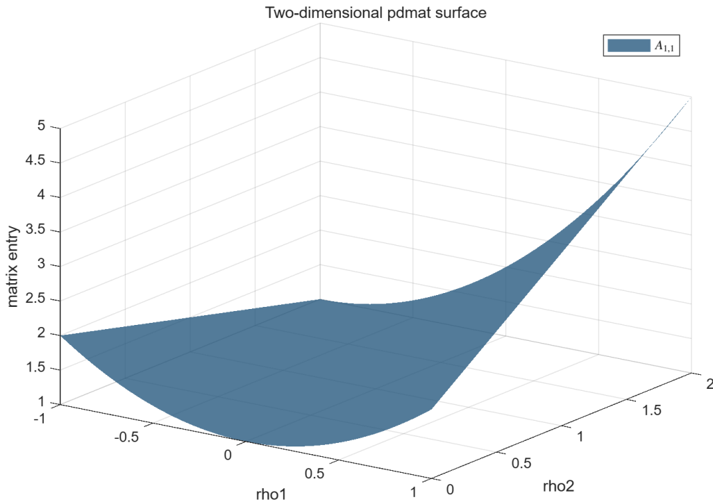
Figure 5.2: Result of the two-dimensional source above.
