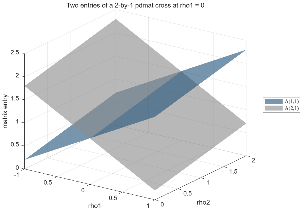
Figure 5.3: Two entry surfaces of a 2-by-1 matrix-valued function. The outside legend distinguishes the entries while their intersection remains visible along \rho_1 = 0 .
