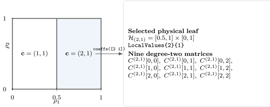
Figure 1.1: A physical hypercube selects one storage leaf. Within that leaf, A2.lbls() supplies the nine zero-based local labels in the displayed order. The matrices are Bernstein coefficients, not a 3-by-3 grid of point samples.
