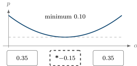
A positive curve can have a negative Bernstein coefficient.
