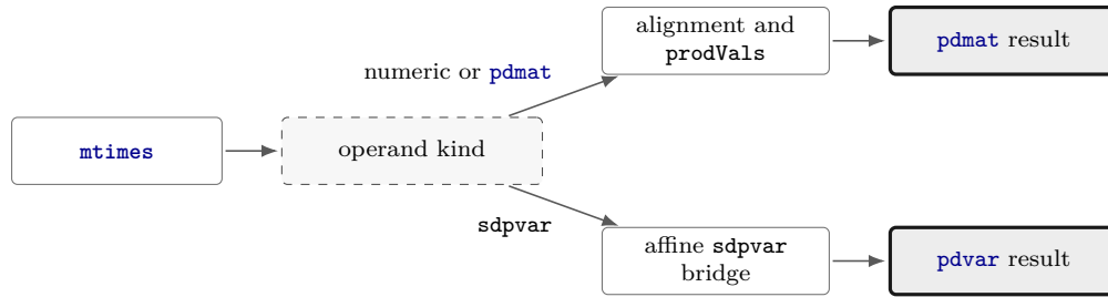
Figure 4.7: Multiplication call paths. Parameter-dependent factors use the ordered binomial-weighted convolution, while a bare affine sdpvar maps the known coefficient tree into pdvar and preserves matrix order.
