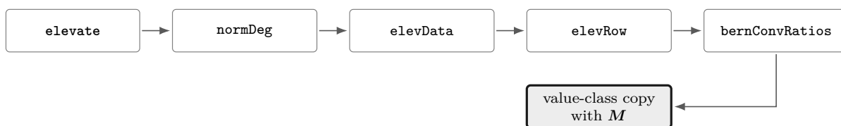
Figure 4.2: Elevation call path. The row kernel reuses exact binomial ratios for every matching source-target degree pair.
