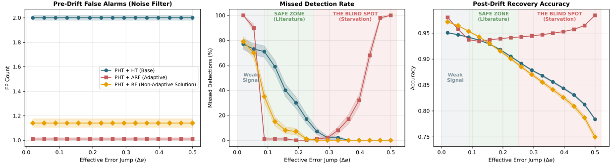
Fig. 3. The Regime Crossover and Architectural Resolution (100 streams/point, bands = \pm 1 SEM). Left (Weak Signal) : models fail to trigger CUSUM. Middle (Safe Zone, \Delta e \approx 0.15 ) : ARF outperforms HT (literature consensus). Right (Blind Spot, \Delta e \geq 0.25 ) : ARF’s hyper-reactive recovery starves the PHT (missed detections climb monotonically across the band, from 1% at its first grid point \Delta e = 0.26 to 100% at \Delta e = 0.50 ). A Non-Adaptive RF (yellow) inherits ARF’s variance reduction (left) while keeping HT’s persistent error signal (right), eradicating starvation (center).
