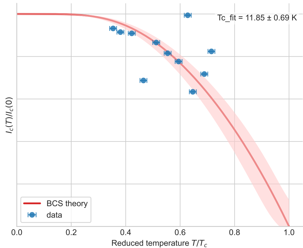
Critical current vs fit T_c
