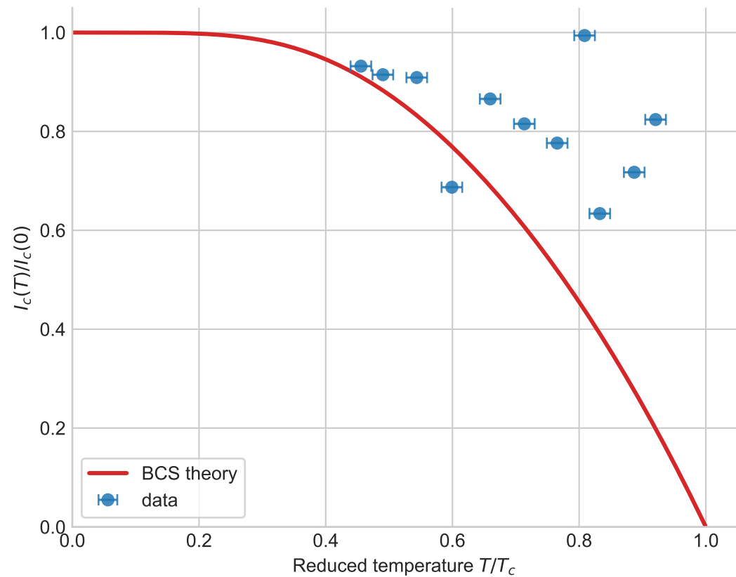
Critical current vs T_c = 9.2 K
