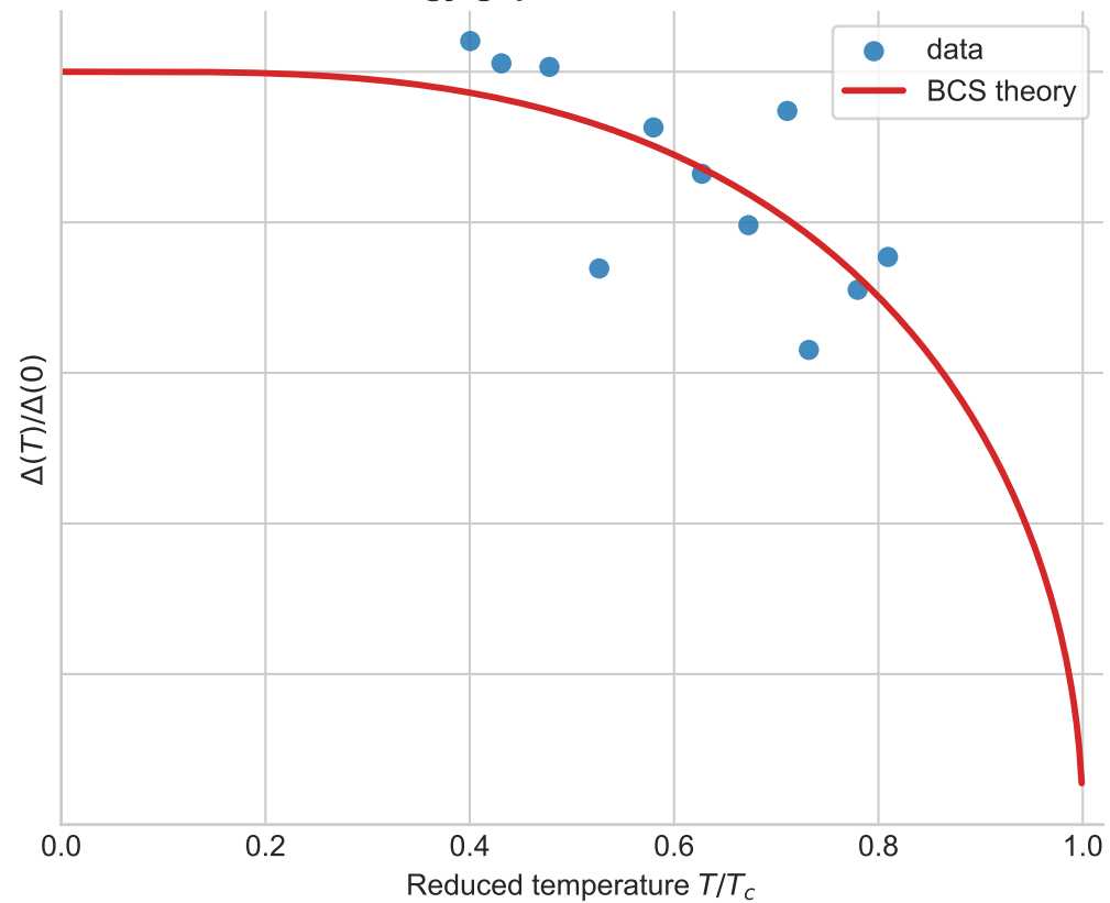
Energy gap vs fit T_c = 10.5 K
