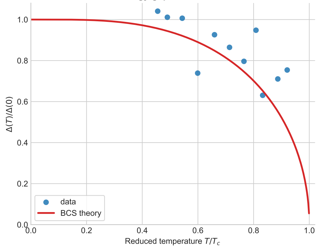
Energy gap vs T_c = 9.2 K
