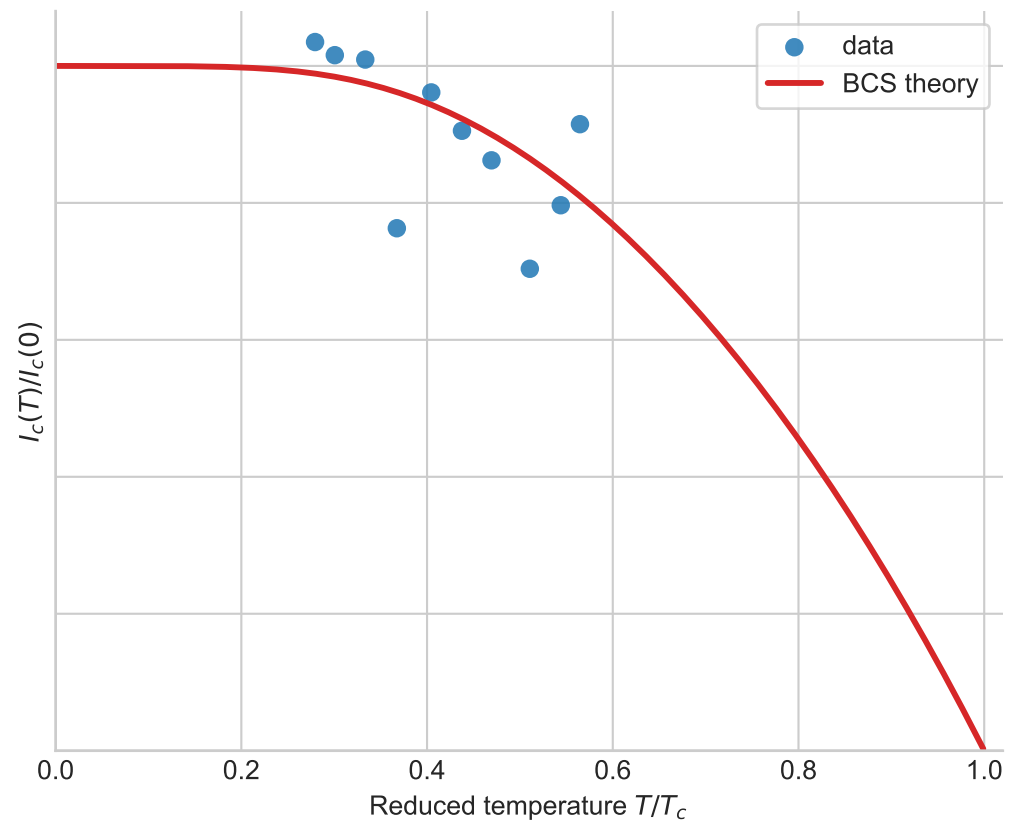
Critical current vs fit T_c = 15 K
