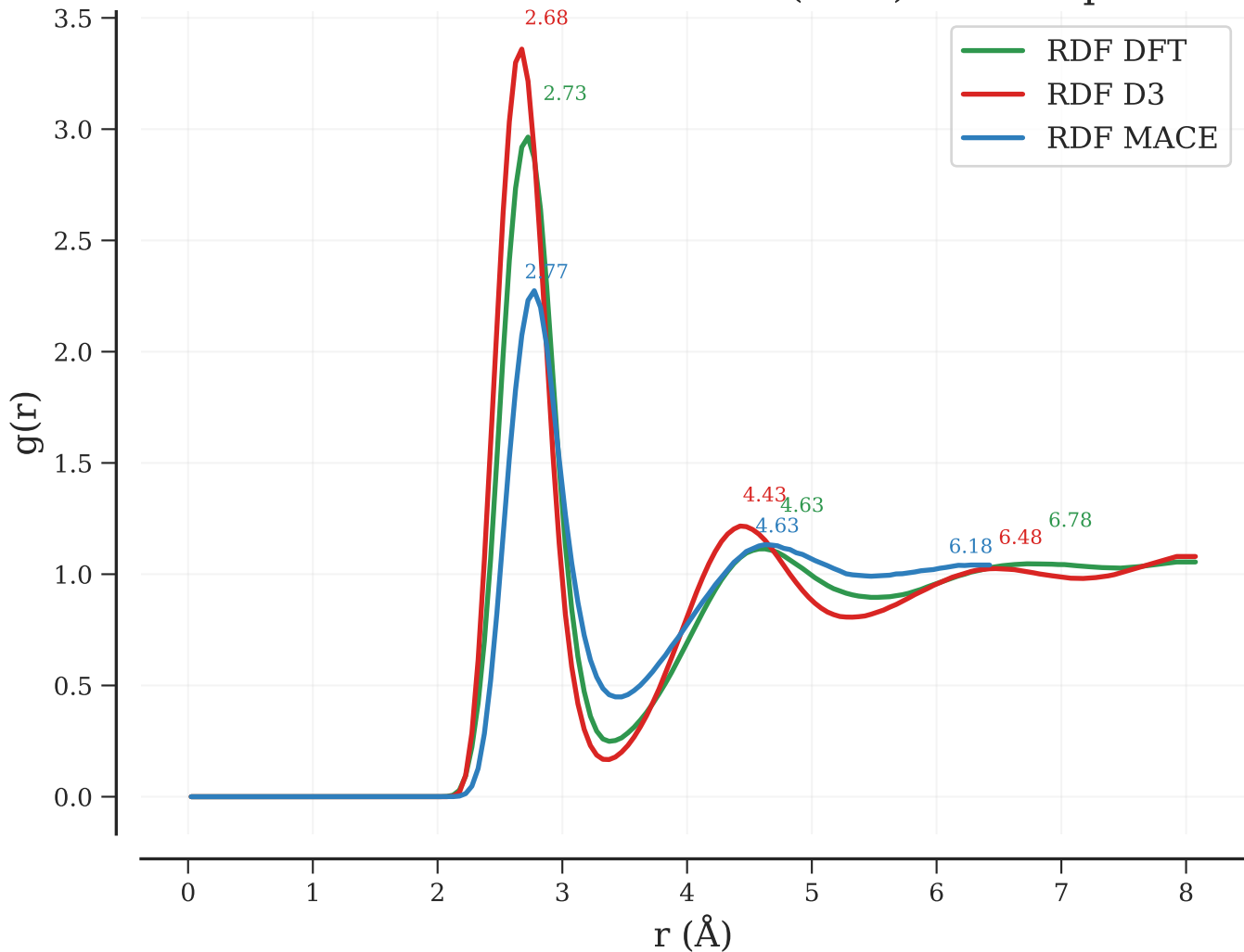
Radial Distribution Function (RDF) for O-O pairs
