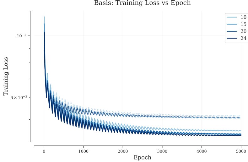
Figure 6: Evaluation of different numbers of basis functions for the MLIP training.
