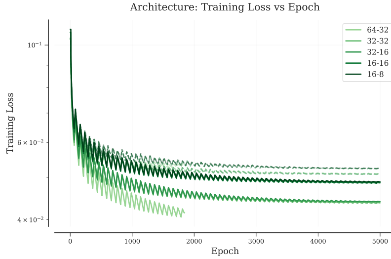
Figure 5: Evaluation of different network architectures for the MLIP training.
