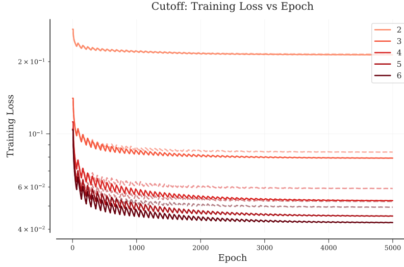
Figure 4: Evaluation of different Radial Cutoff ( r_{max} ) for the MLIP training.
