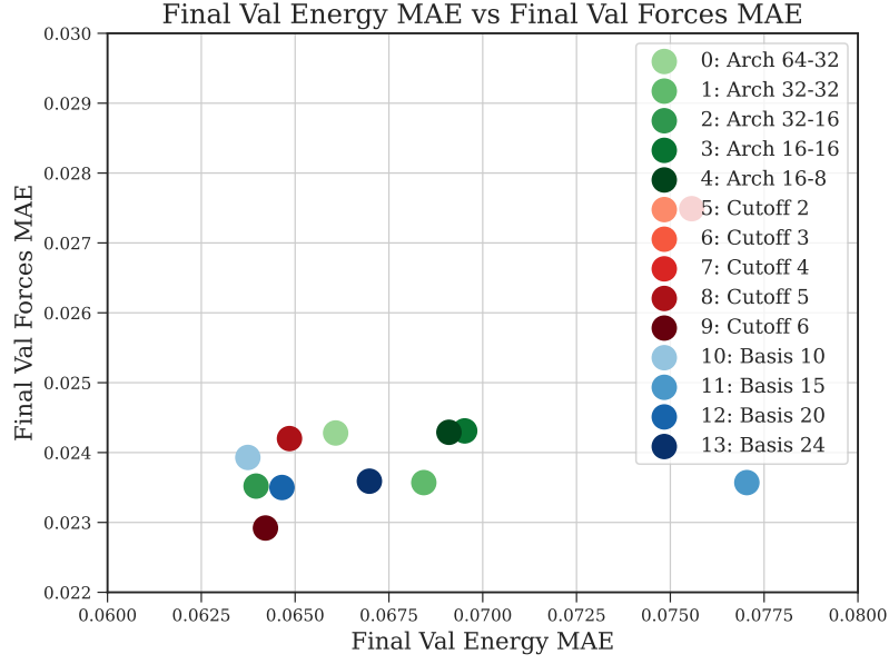
Figure 7: Evaluation of different neural network hyperparameter. The plot only compares the final force and energy MAE, not the final training loss.
