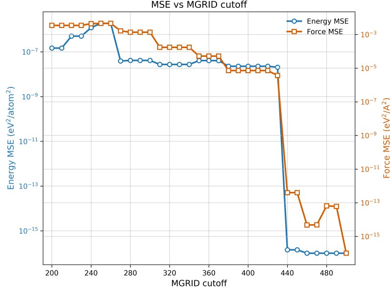
Figure 3: Evaluation of the mgrid cutoff parameter for DFT settings for the PBE functional in CP2K calculation.
