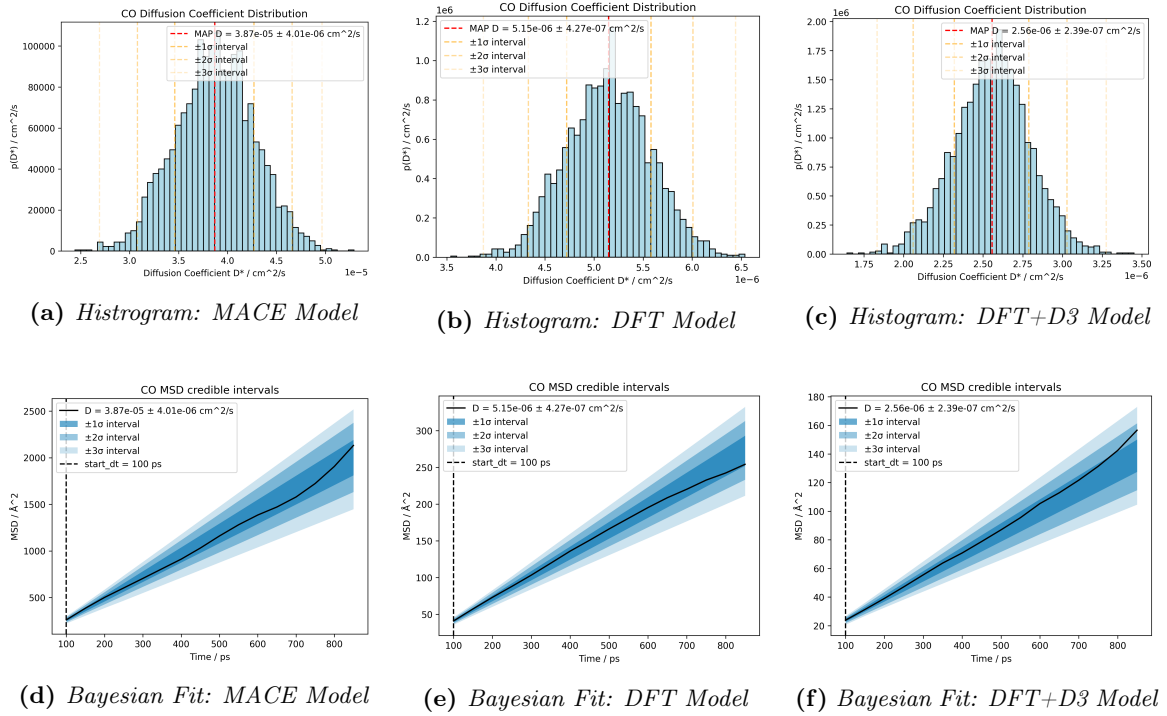
Figure 8: Evaluation of the self diffusion coefficient of the production MD simulations for three different models: MACE, PBE, PBE+D3 dispersion correction.
