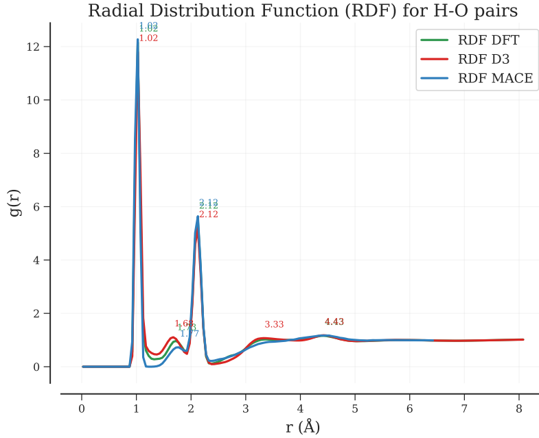
Figure 9: Radial distribution function of three models compared for the O-H bonds.
