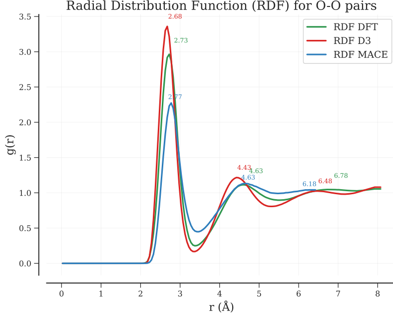
Figure 10: Radial distribution function of three models compared for the O-O bonds.
