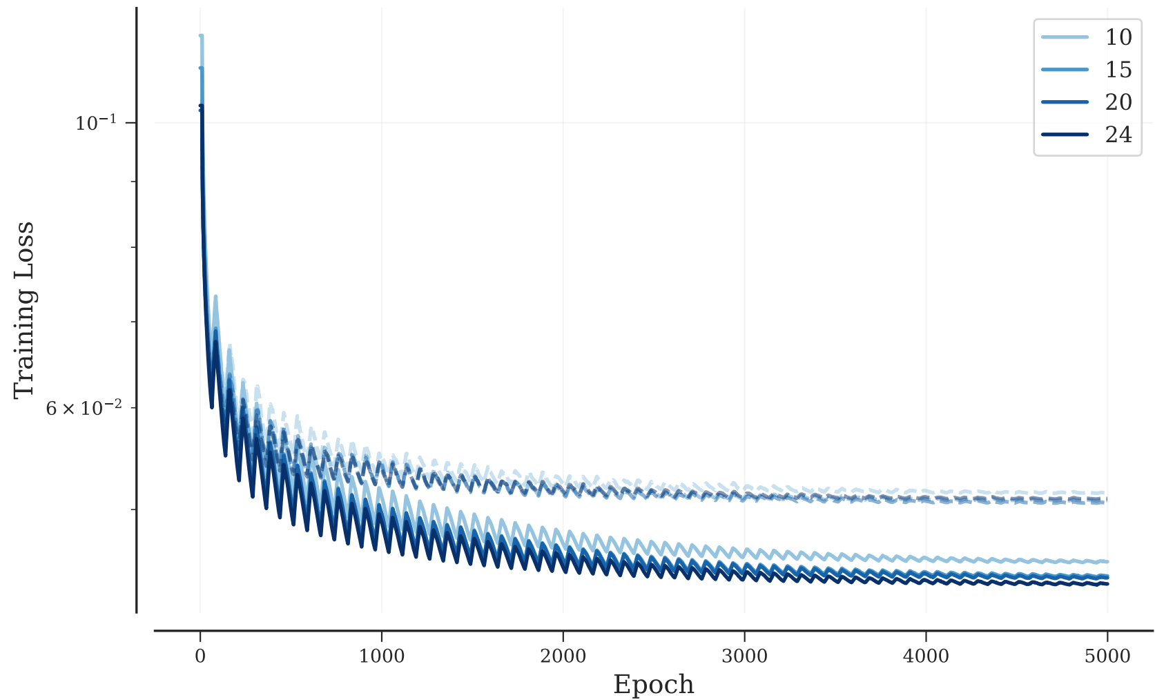
Basis: Training Loss vs Epoch
