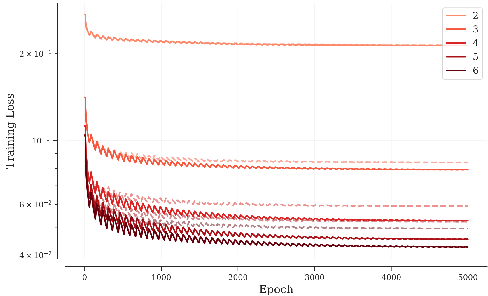
Cutoff: Training Loss vs Epoch
