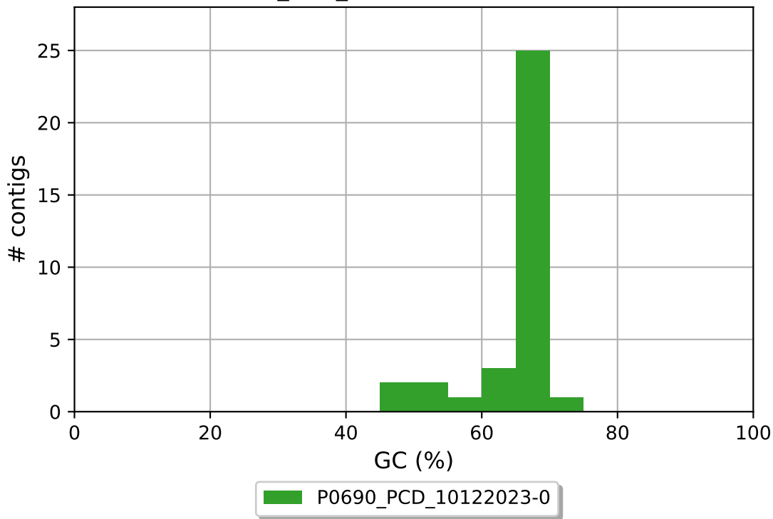
P0690_PCD_10122023-0 GC content
