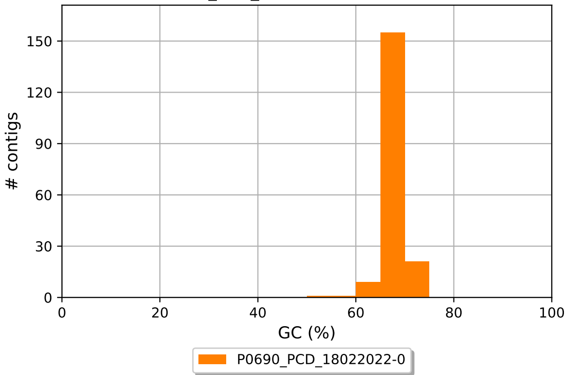
P0690_PCD_18022022-0 GC content
