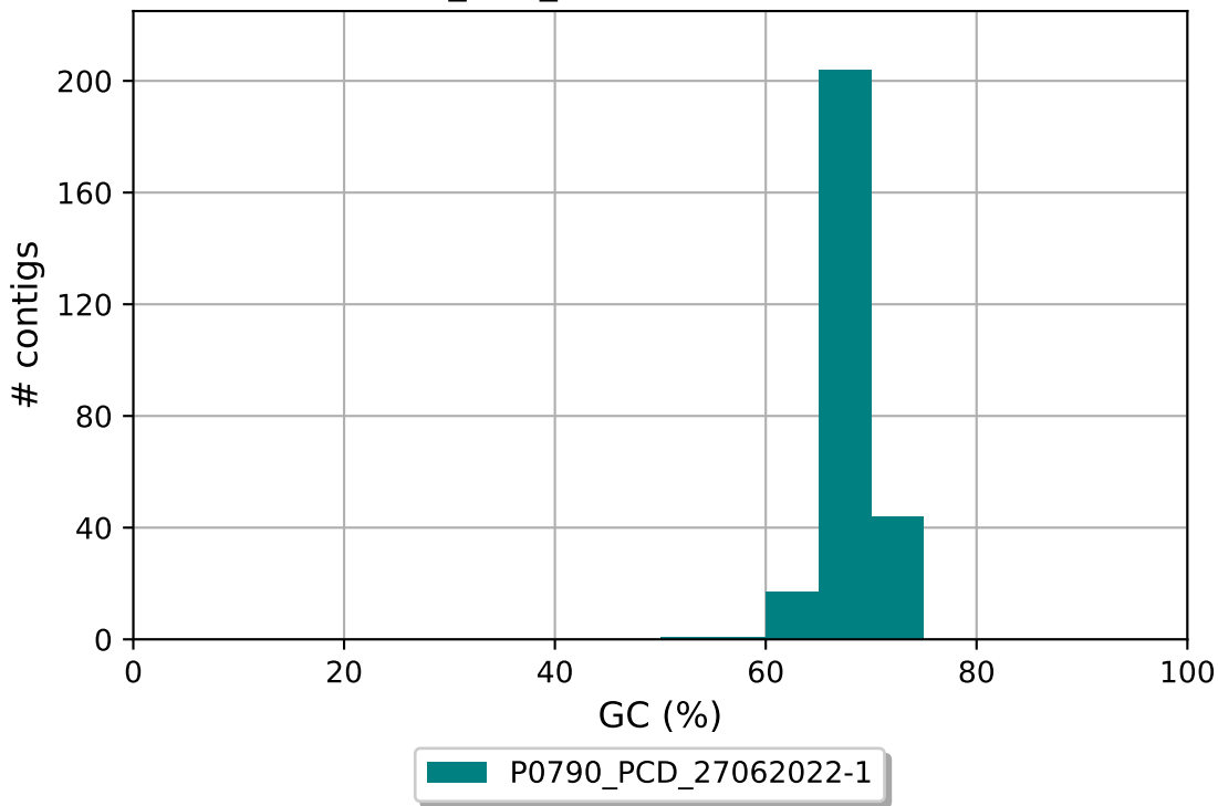
P0790_PCD_27062022-1 GC content
