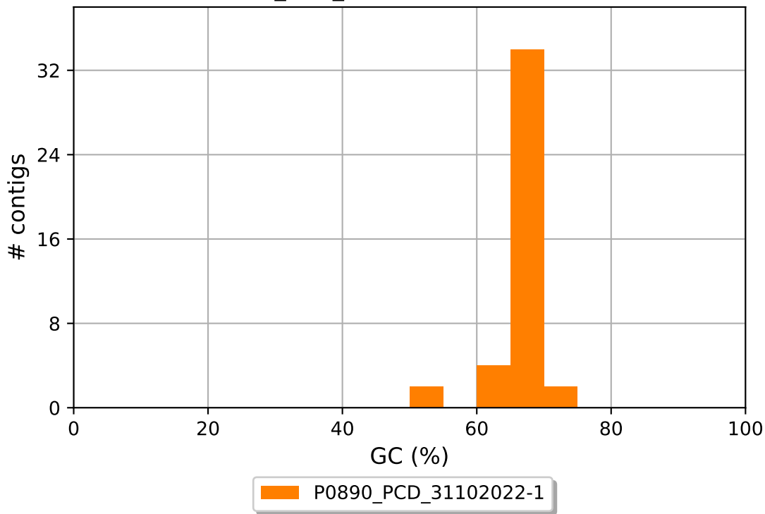
P0890_PCD_31102022-1 GC content
