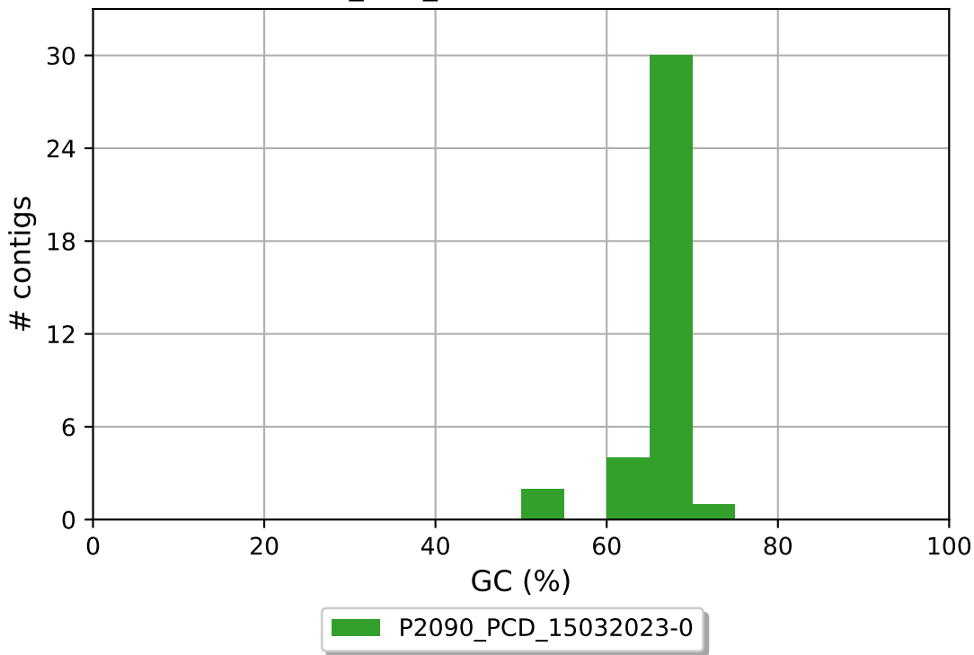
P2090_PCD_15032023-0 GC content
