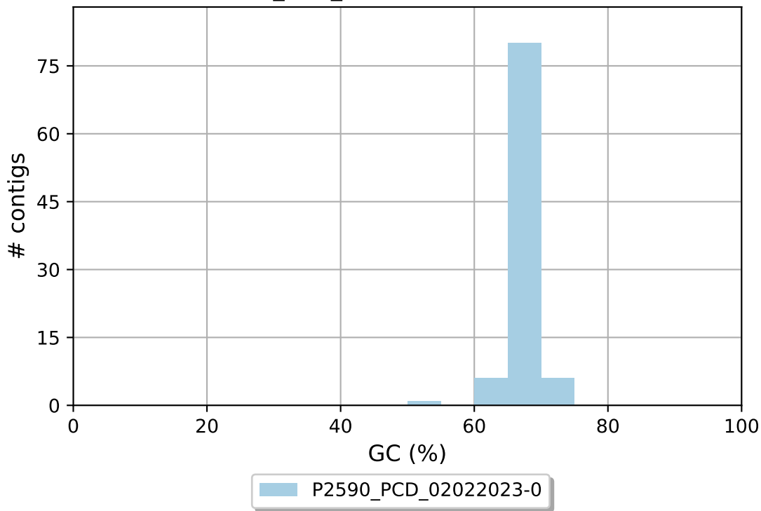
P2590_PCD_02022023-0 GC content
