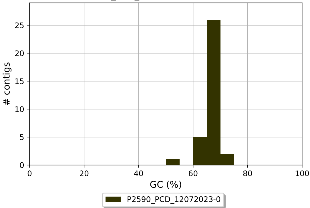
P2590_PCD_12072023-0 GC content
