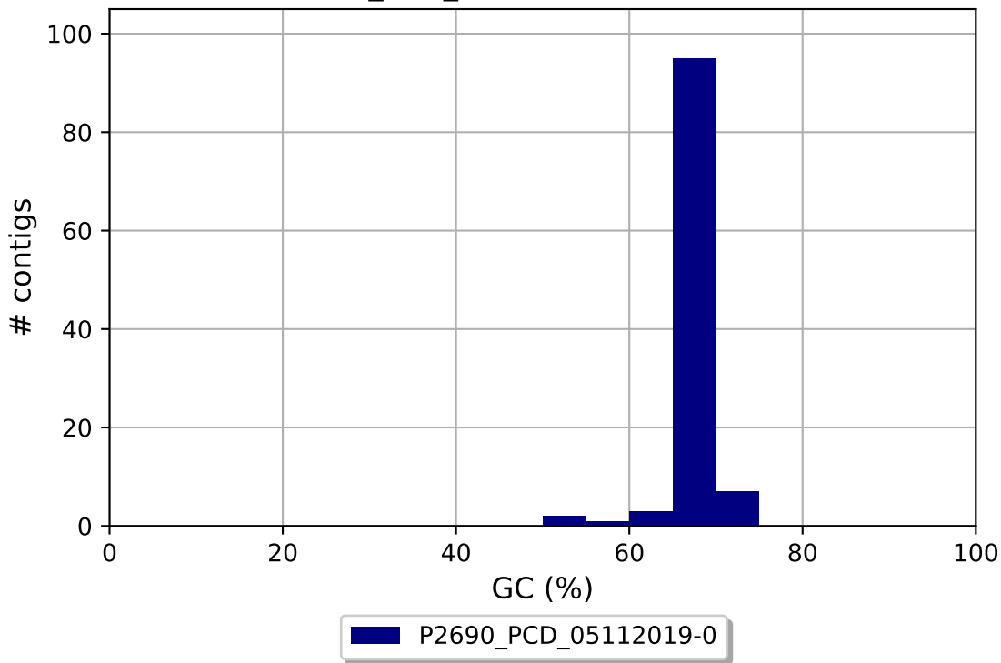
P2690_PCD_05112019-0 GC content
