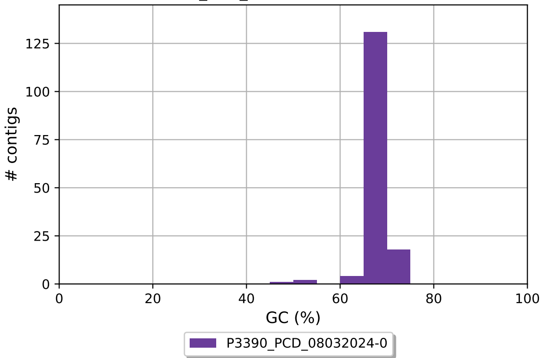
P3390_PCD_08032024-0 GC content
