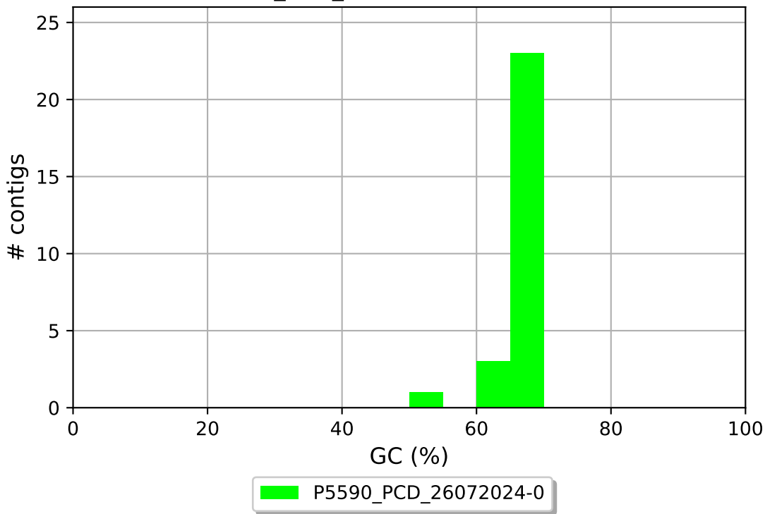
P5590_PCD_26072024-0 GC content
