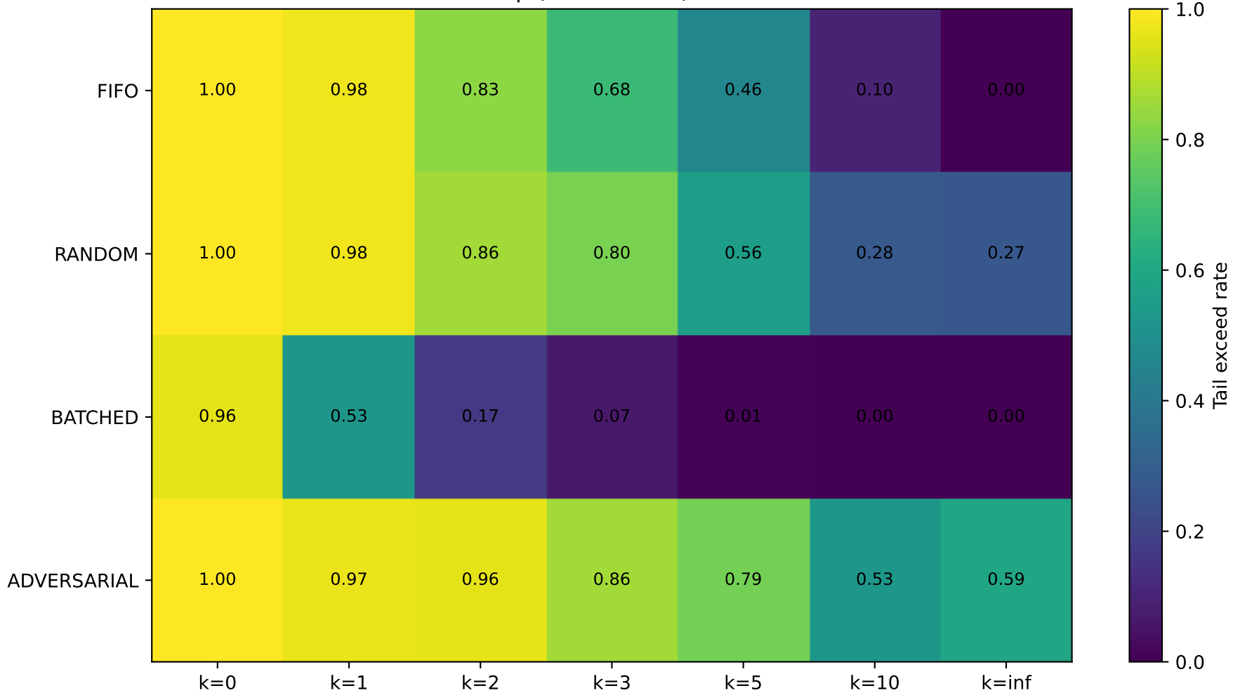
Risk-Cliff Heatmap (fault=NONE) — Tail exceed rate
