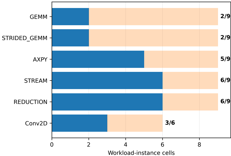
(a) Conflicts by workload family
