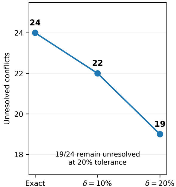
(b) Conflict hardness
