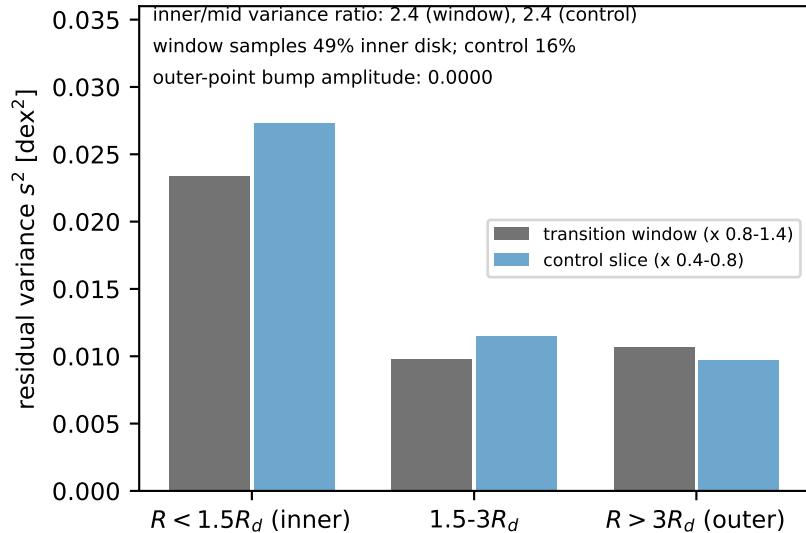
(b) the transition excess is inner-disk structure
