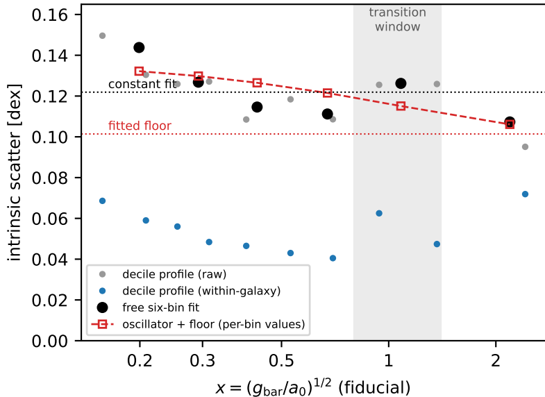
(a) the scatter is acceleration-dependent
