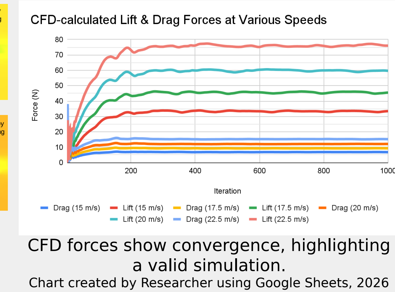
Fig 2. CFD-Calculated Forces
