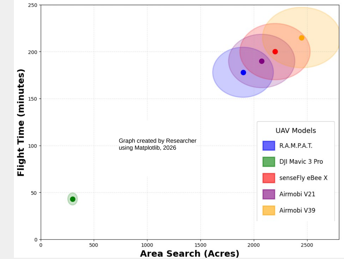
UAV Performance with Error Propagation
