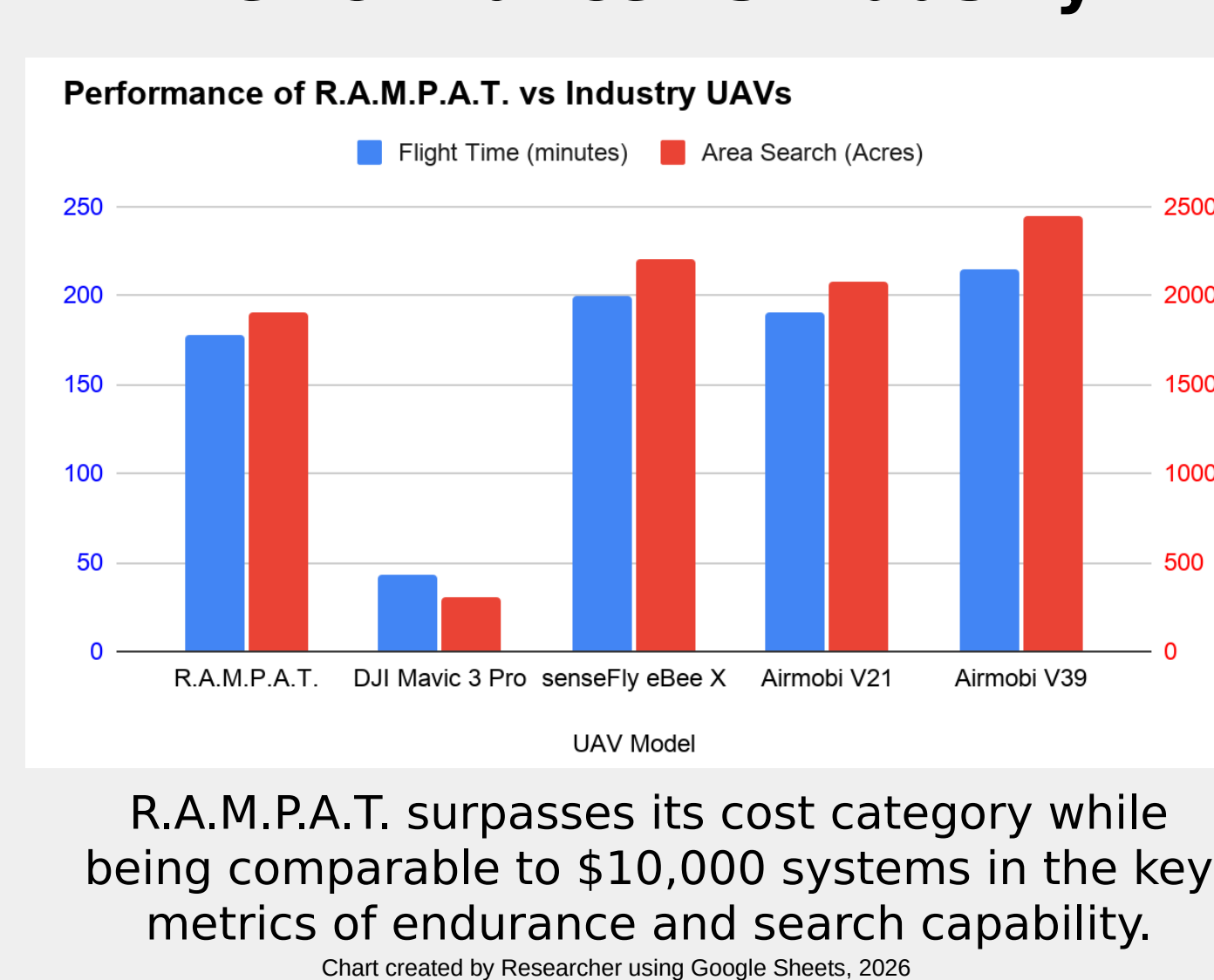
Fig 6. R.A.M.P.A.T. Performance vs Industry
