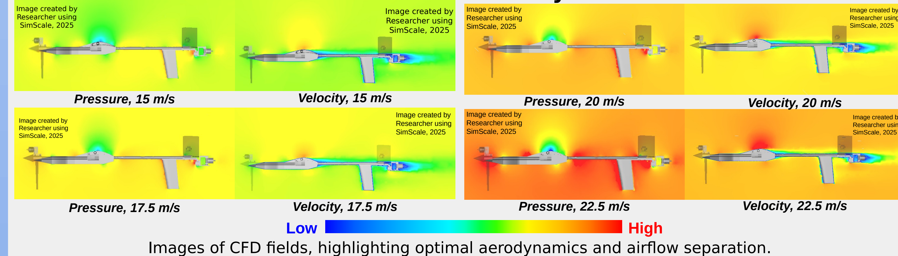
Fig 1. Airflow Property Fields of R.A.M.P.A.T. Geometry
