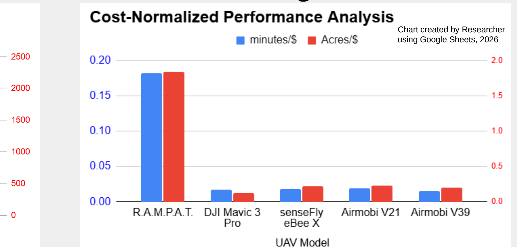
Fig 7. Cost-Normalized Performance of R.A.M.P.A.T. vs Existing UAVs
