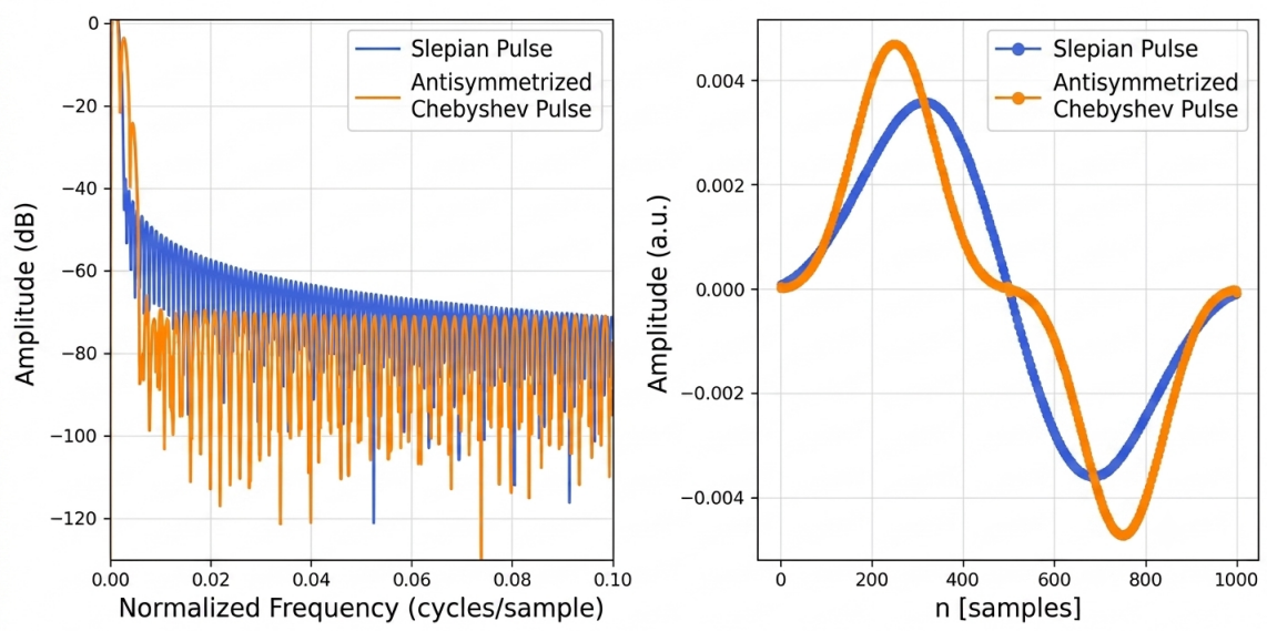
Figure 1: The parameter r is chosen so that sidelobe height is 40 dB lower than the first slepian sidelobe height.
