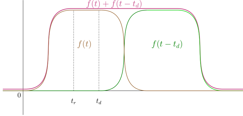
Figure 2: Creating a flat-top pulse using echo method
