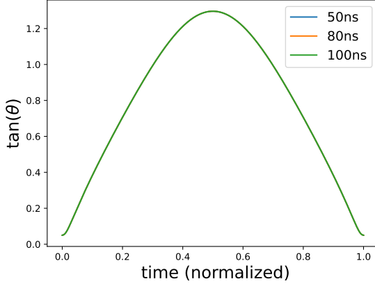
Figure 5: The relation between \tau and t for the Slepian pulse with N = 50 , \Delta = 0.8 , and T = 100 . The three graphs are overlapping each other due to almost the same A(\tau_d) .
