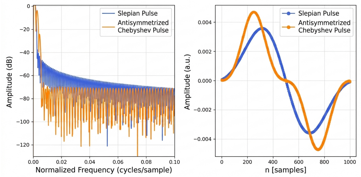
Figure 4: The parameter r is chosen so that sidelobe height is 40 dB lower than the first slepian sidelobe height.
