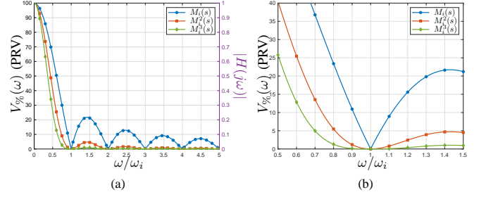
Fig. 3. Percentage Residual Vibration (PRV)/Frequency response of rectangular smoothers M_k(s) , k = 1, 2, 3 as a function of the normalized frequency \omega/\omega_i (a) and magnification in the neighborhood of the first zero (b).
