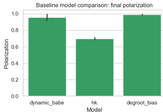
Figure 6: Final polarization under Dynamic-BABE Baseline, Hegselmann–Krause, and biased DeGroot-style updates (20 seeds).
