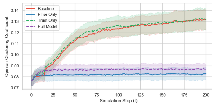
Figure 4: Opinion-weighted clustering (local active-triple average). Filter ON conditions reduce local same-pole triangles relative to Baseline while active-agent polarization remains high. Error ribbons: 95% CIs.
