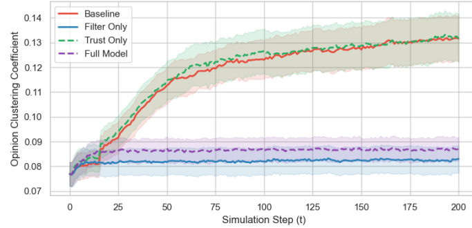
Figure 4: Opinion-weighted clustering (local active-triple average). Filter ON conditions reduce local same-pole triangles relative to Baseline while active-agent polarization remains high. Error ribbons: 95% CIs.
