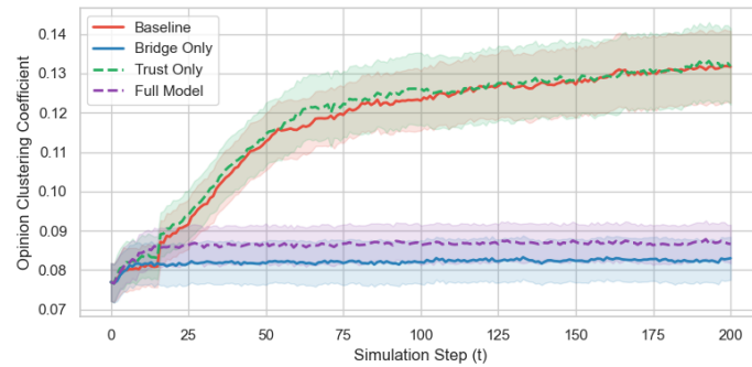
Figure 4: Emergent structural echo chambers, measured via the opinion-weighted clustering coefficient over time (active triples only). The suppression filter (Bridge Only and Full Model) significantly reduces local triadic homogeneity compared to the Baseline, although global active-agent polarization remains extreme. Error ribbons show 95% confidence intervals.
