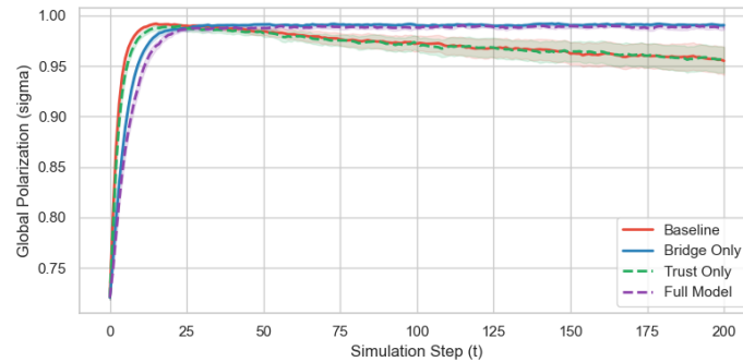
Figure 2: Active-agent opinion polarization ( \sigma ) over time across the four experimental conditions. While the suppression filter reduces churn in the Bridge Only condition, it paradoxically locks systemic polarization at a significantly higher level ( \sigma \approx 0.9904 ) compared to the Baseline ( \sigma \approx 0.9550 ), demonstrating the Polarization Paradox. Error ribbons represent 95% confidence intervals.
