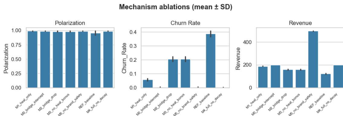
Figure 5: Mechanism ablations (20 seeds): mean Polarization, Churn Rate, and Revenue by condition. Error bars show standard deviations.
