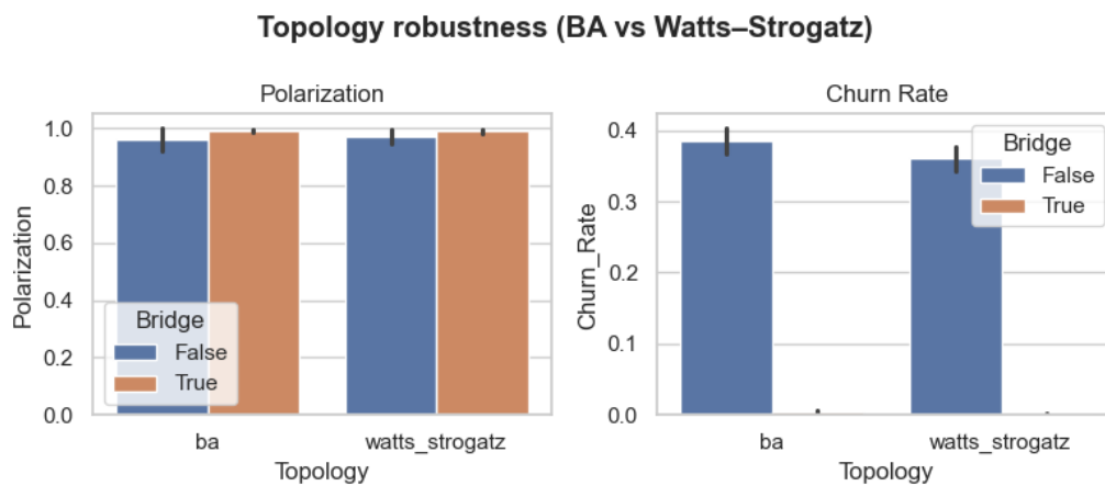
Figure 7: Bridge OFF/ON contrasts on Barabási–Albert vs. Watts–Strogatz topologies (15 seeds).
