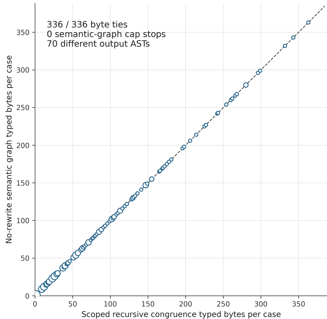
Representation comparison on the held-out corpus
