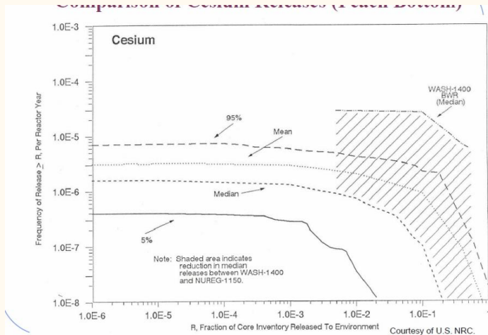
Figure. cesium release to environment
