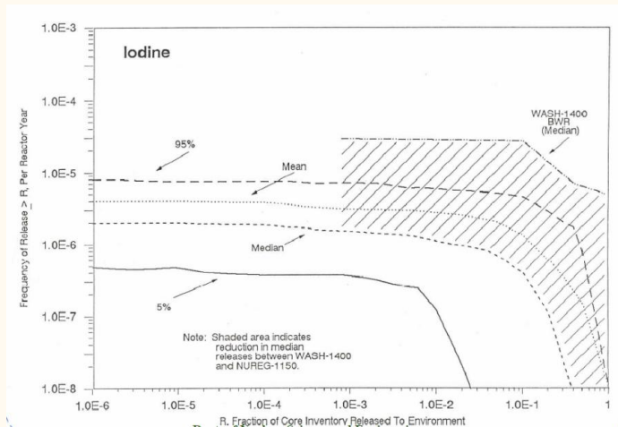
Figure. Iodine release to environment
