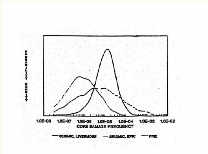
Figure. Core damage frequency for earthquake and fire
