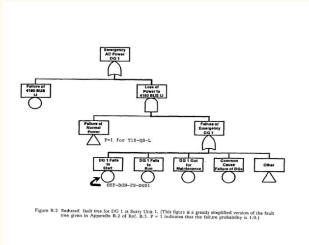
Figure. Fault tree from the WASH-1400 report
