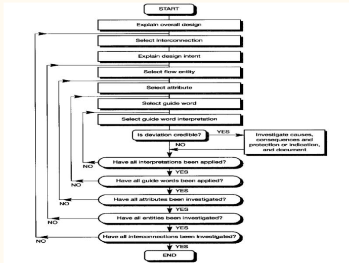
Figure. Basic HAZOP flowchart
