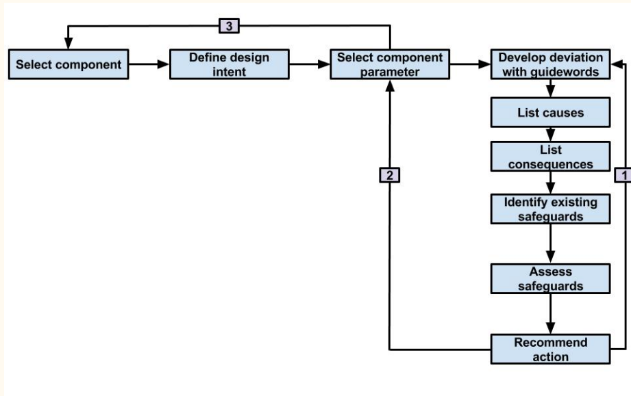
Figure. HAZOP design loop
