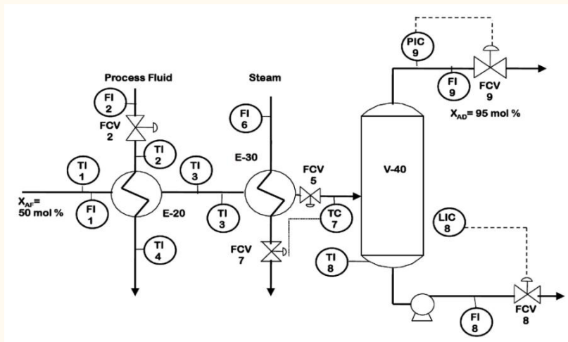
Figure. HAZOP flash drum example. More slides in the OER
