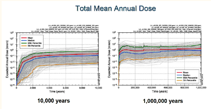
Figure 24: Yucca Mountain expected annual dose for ten thousand and one million years
