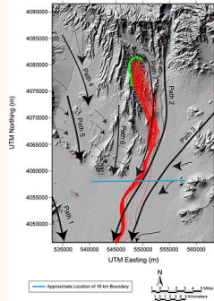
Figure 25: Groundwater flow from Yucca Mountain
