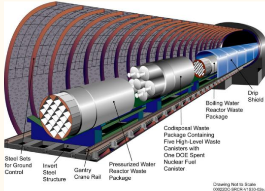
Figure 22: Yucca Mountain tunnel design
