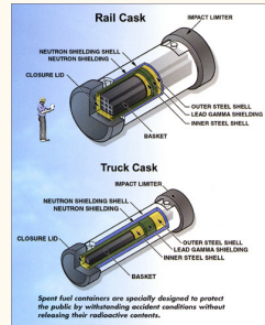
Figure 5: SNF transport casks
