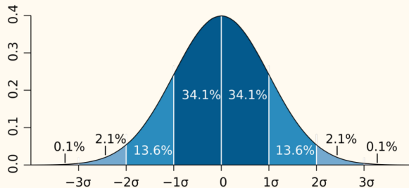
Figure. Example normal distribution
