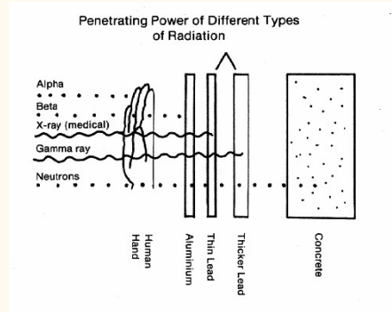
Figure 11. Radiation shielding materials
