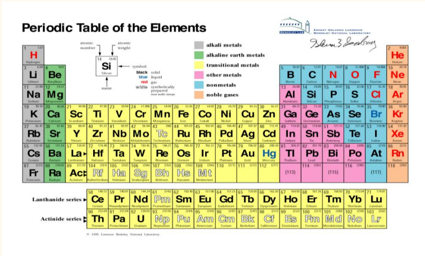
Figure 5. Periodic table of the elements
