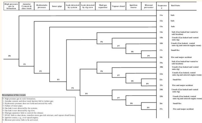
Figure. Event tree for fracking accidents
