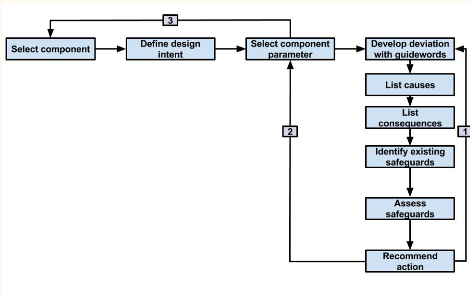
Figure. HAZOP design loop
