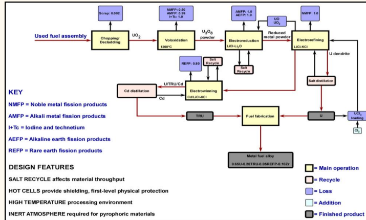
Figure 8: Pyroprocessing flowsheet
