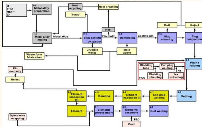
Figure 3: Fuel fabrication process steps
