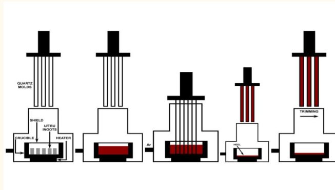
Figure 2: Metal fuel assembly process
