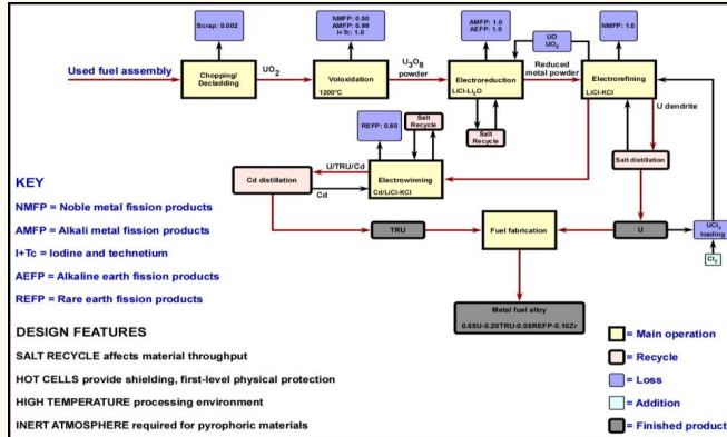
Figure 1: Pyroprocessing flowsheet
