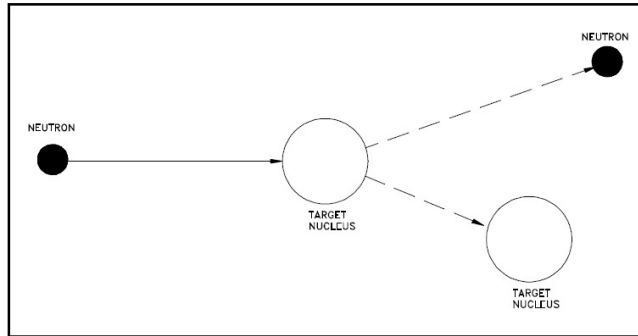
Figure 16 Elastic Scattering
