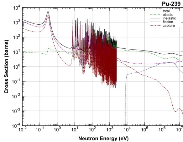
Figure 13: Pu239 cross sections
