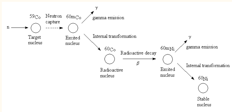
Figure 9: Neutron capture
