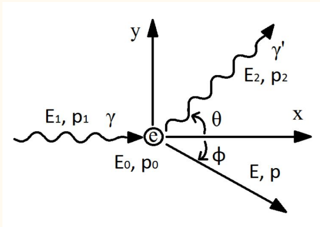
Figure 3: Compton effect
