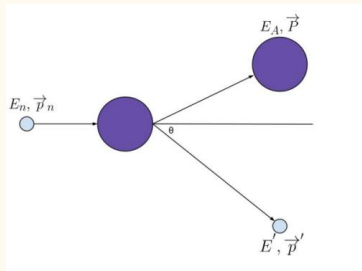
Figure 7: Elastic scattering
