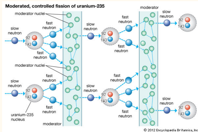
Figure 4: Fission
