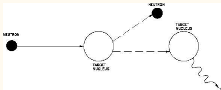
Figure 8: Inelastic scattering
