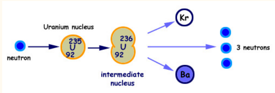
Figure 5: Compound nucleus
