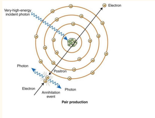
Figure 2: Pair production
