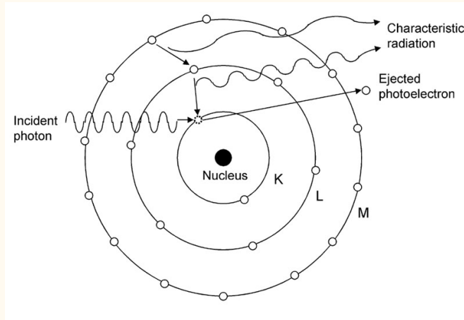
Figure 1: Photoelectric effect
