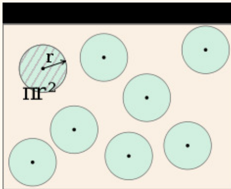
Figure 10: Cross sections
