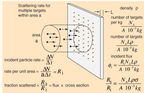
Figure 15: Neutron flux
