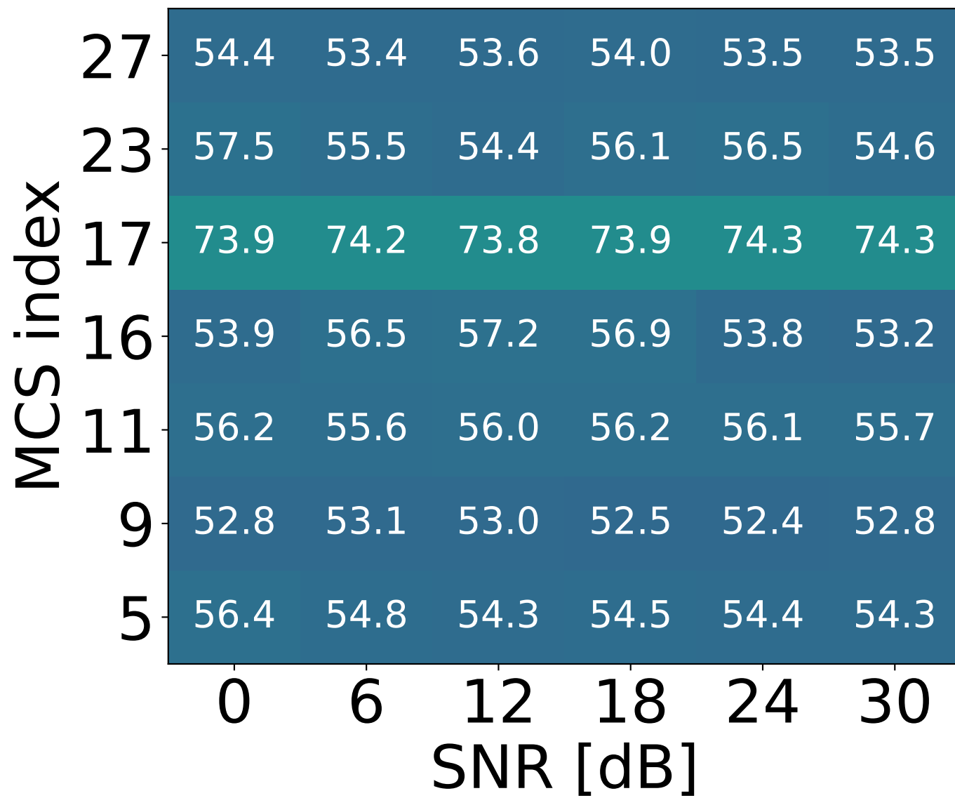
GPU 1 CB
