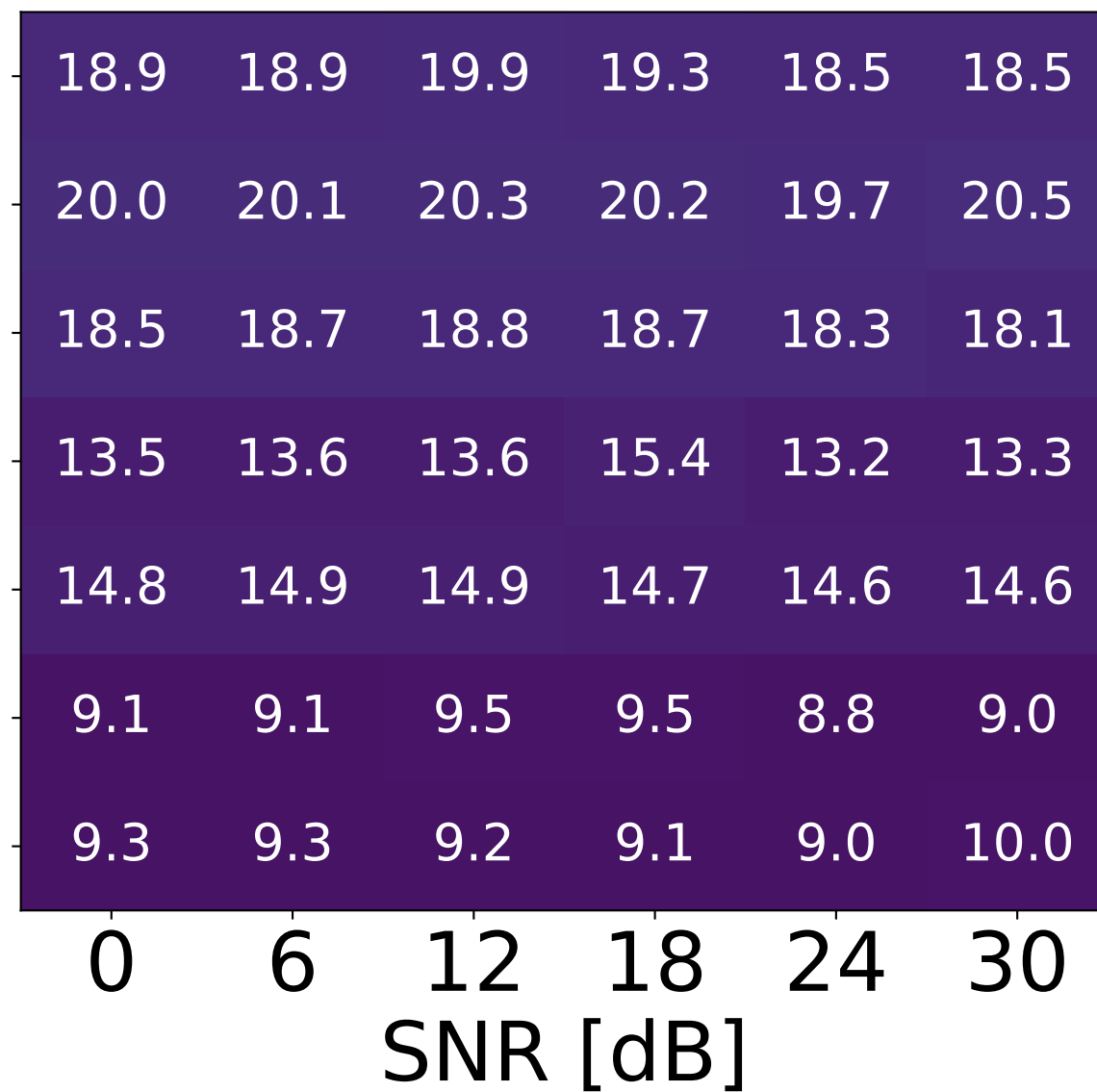
GPU 1024 CBs + bus
