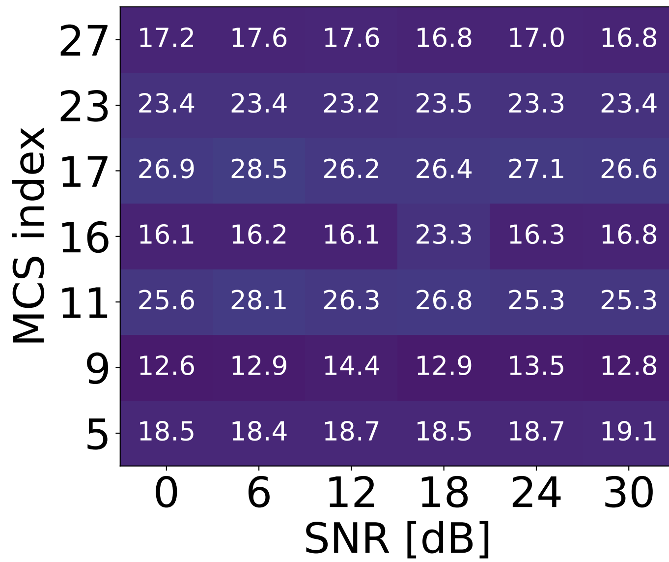
CPU
