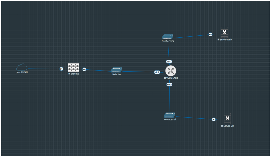
Figure 7.4: Lab 3 network topology
