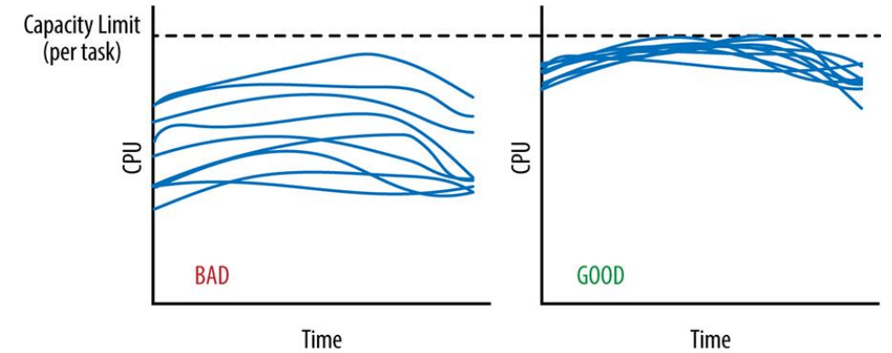
CPU Usage by Task at a Given Time
