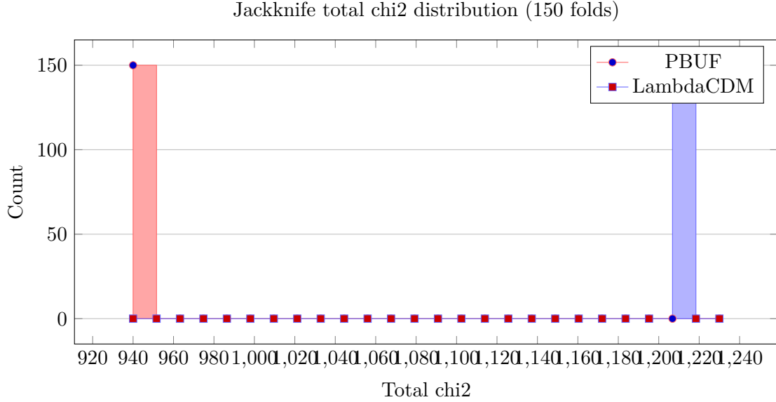
Figure 2: Histogram of total chi2 across 150 jackknife folds for PBUF and LambdaCDM.
