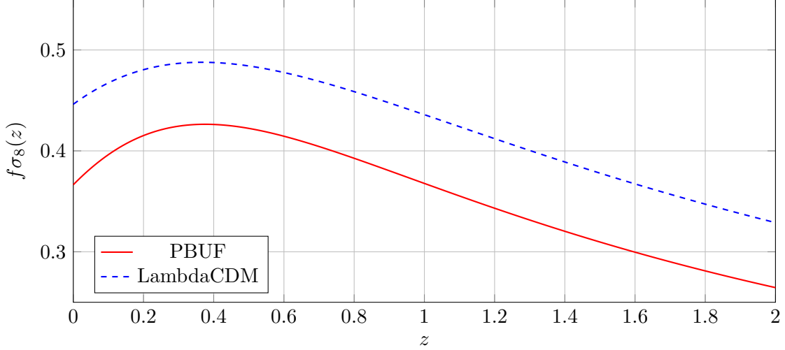
Figure 5: Predicted f\sigma_8(z) trajectory versus the LambdaCDM baseline.
