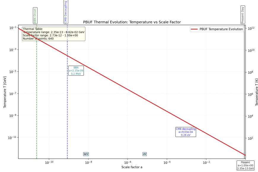
Figure 1: Thermal lookup-table trajectory produced by the LUT referenced in this section; the same curve seeds the expansion and growth predictions introduced later.
