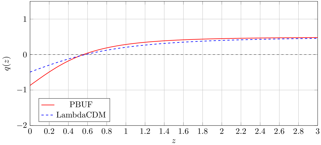
Figure 4: Predicted deceleration history in PBUF compared to the LambdaCDM baseline.
