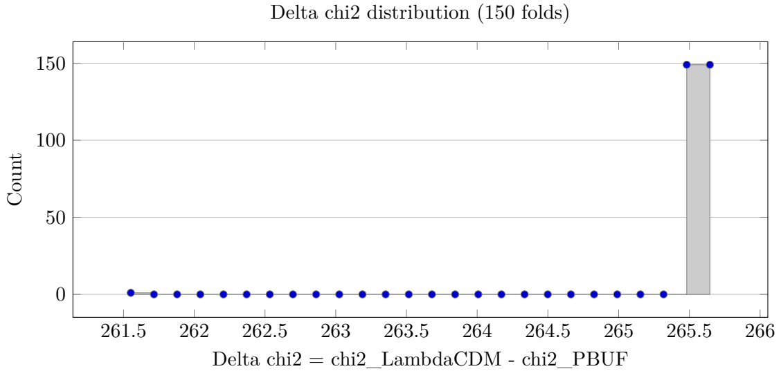
Figure 3: Histogram of Delta chi2 across 150 jackknife folds. All values are positive in this run set.
